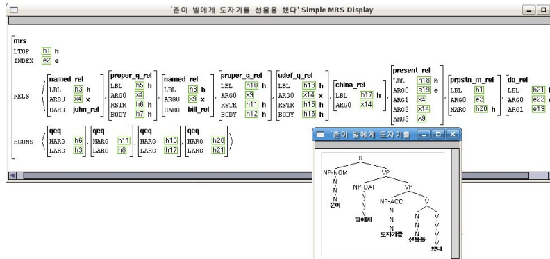
Figure 1: Parsed Tree and MRS for (9a)
