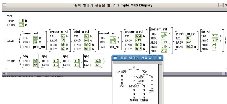
Figure 2: Parsed Tree and MRS for (25a)
